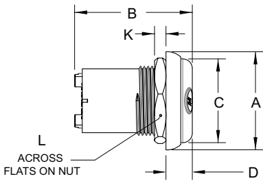
[E] RECEPTACLE
